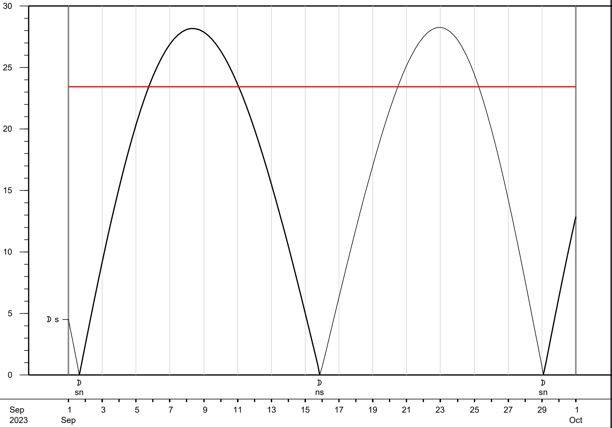
Declination Graph Geocentric Transits from Sep 1 2023 AD GC 12:00:00 AM CDT +05:00:00
